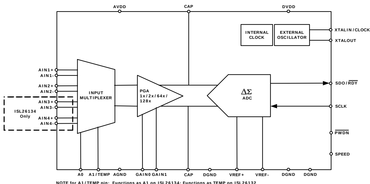
FIGURE 1. BLOCK DIAGRAM
